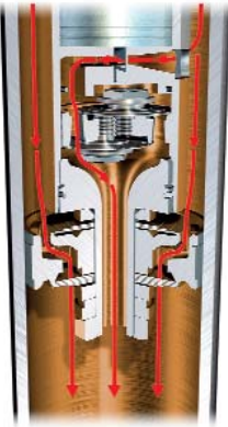
Rebound in 'Normal' mode – bypass valve open
