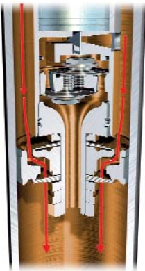
Rebound in 'Sport' mode – bypass valve closed
