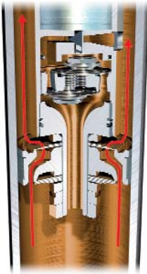
Compression in 'Sport' mode – bypass valve closed
