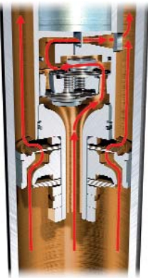
Compression in 'Normal' mode – bypass valve open
